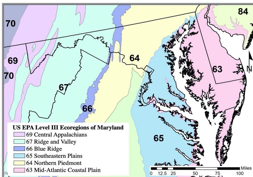
Fig. 1. EPA Level III Ecoregions of Maryland.
